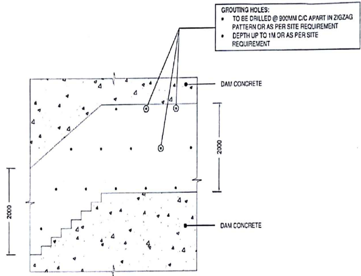
LONGITUDINAL SECTION OF INSPECTION GALLERY
