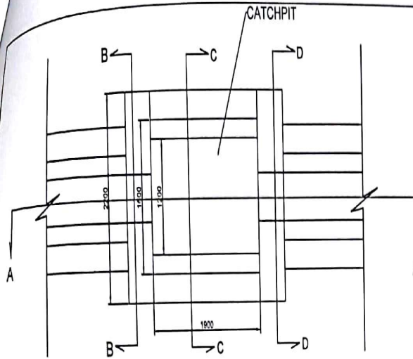
FIG: PLAN OF CATCHPIT
